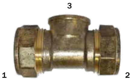
PLCX0027 Tee 15mm CxFI
